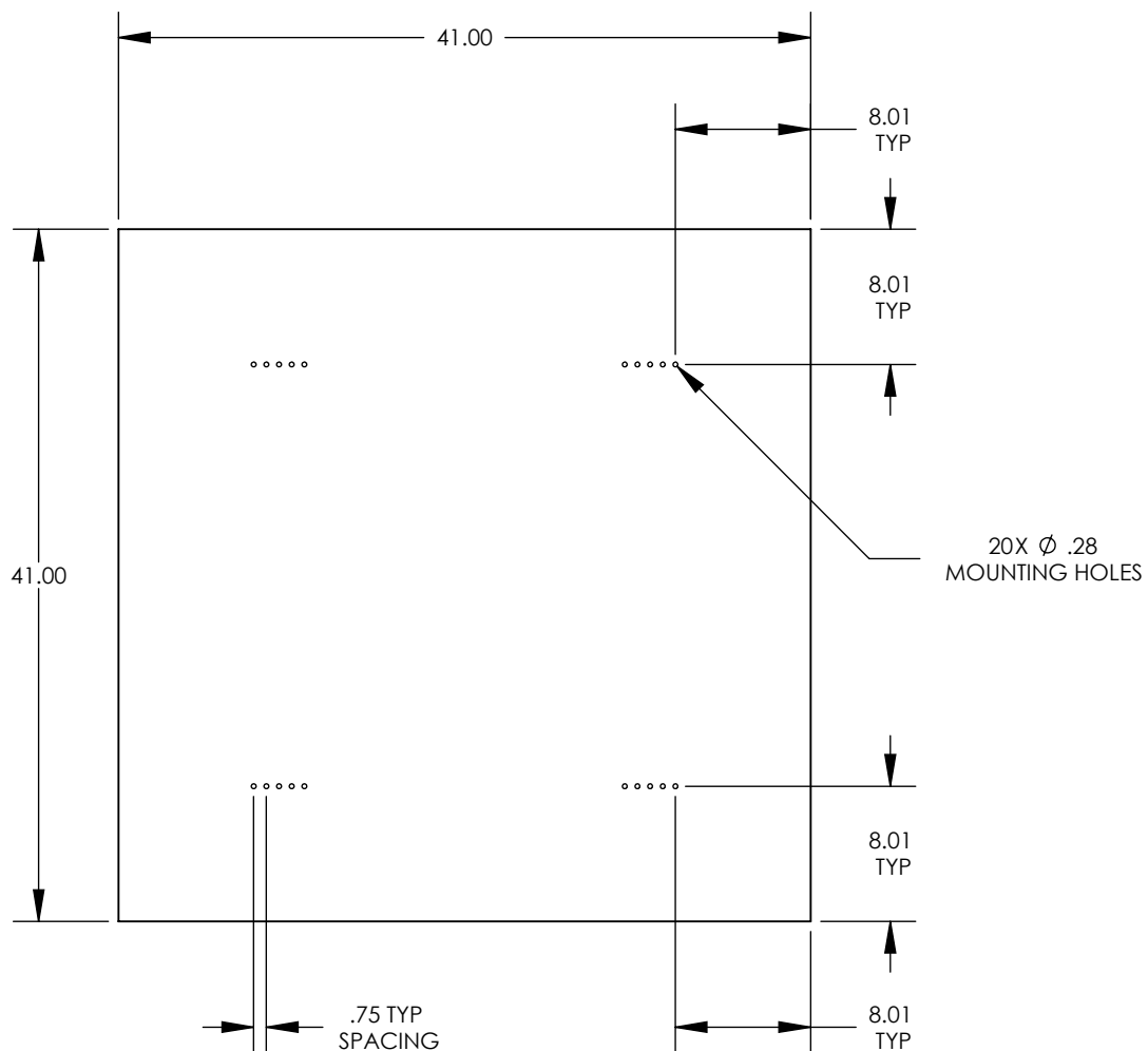
WALL MOUNTING DETAIL
